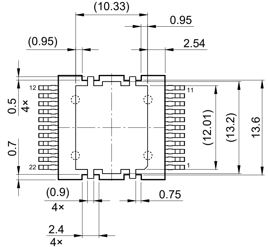
Bottom view
