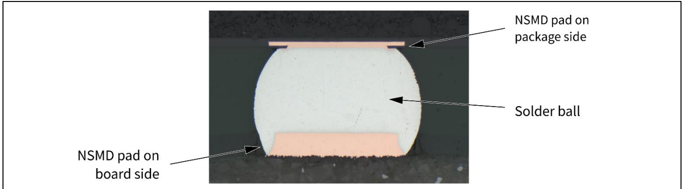
Figure 10 Cross-section of an eWLB solder ball with NSMD pad on the component side and NSMD pad on the board side. The latter allows the solder to “grip” the pad sidewalls increasing the board level reliability of the component.
