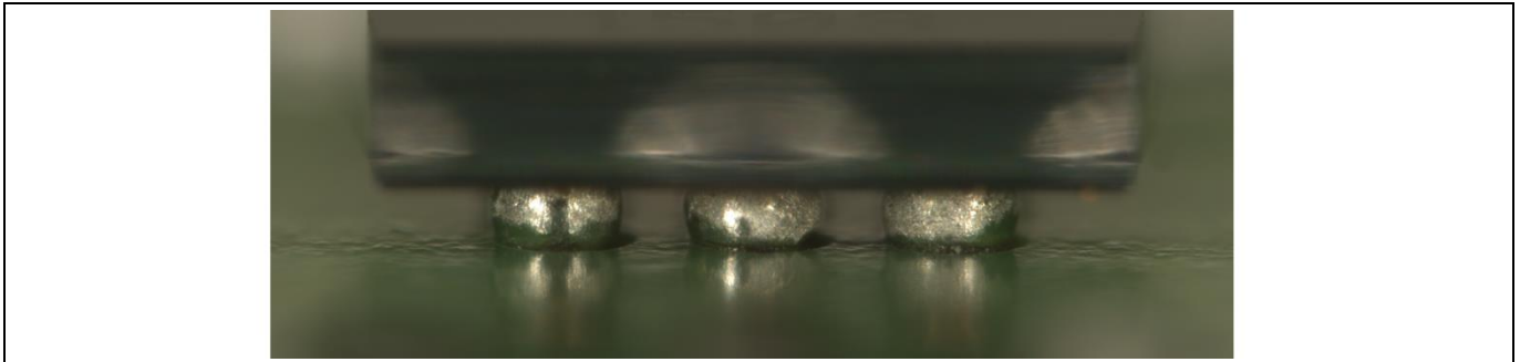
Figure 12 Side view of a WLB package mounted on NSMD PCB pads. The component silicon body and the solder ball terminals can be seen from top to bottom.
