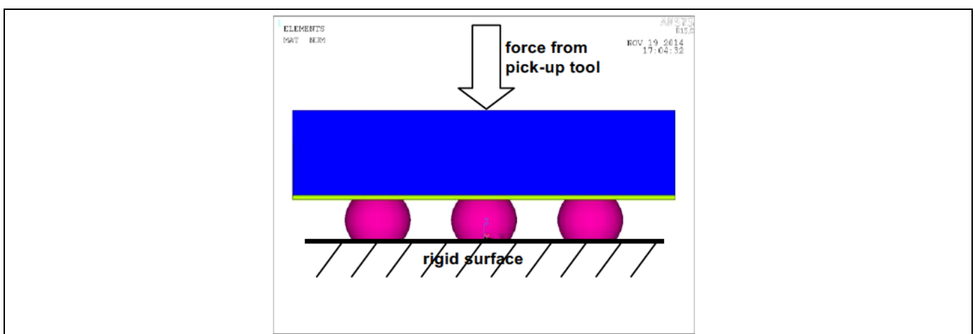
Figure 11 Schematic of the simulation model for nozzle pick force assessments.
