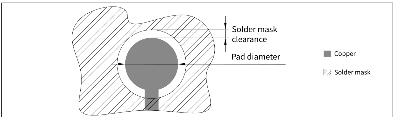
Figure 9 Recommended NSMD PCB pad design. Pad diameter and solder-mask clearance depend on the individual components, and can be found in the Infineon package data base that is available on the Infineon web page [1].
