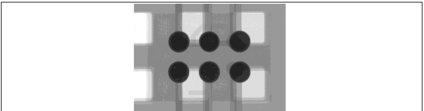
Figure 13 X-ray photograph of a properly soldered WLB component. The solder balls and the RDL lines are visible.
