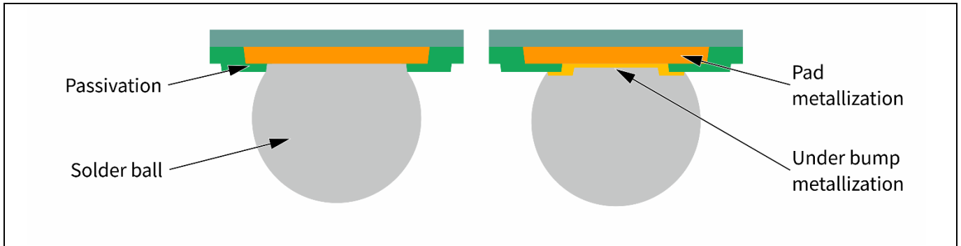
Figure 8 Schematic comparison of a typical SMD ball pad (left) on WLB components and a NSMD ball pad (right) on eWLB components.
