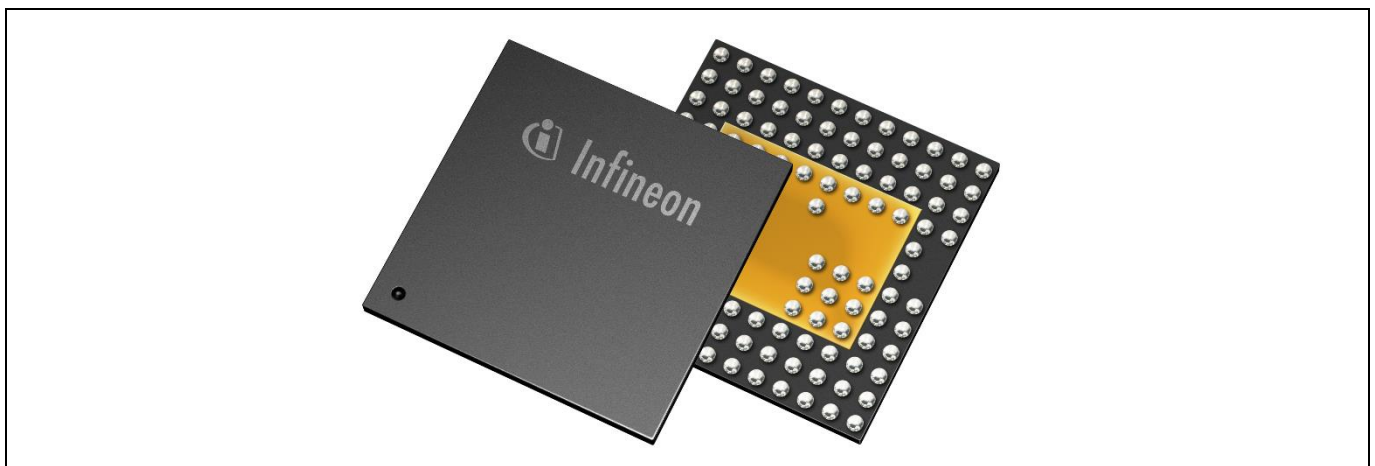
Figure 3 Example of embedded WLB packages.
