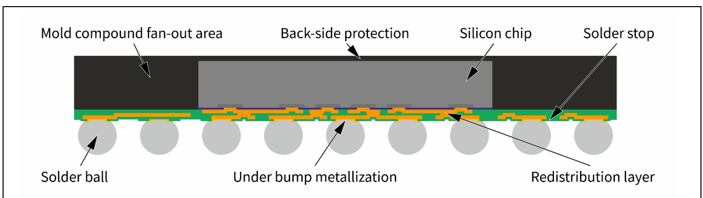
Figure 7 Schematic of the inner setup of typical eWLB components.
