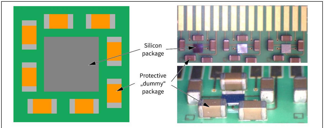
Figure 4 Schematic top view and photographs of showing passive components surrounding a silicon package for mechanical protection.
