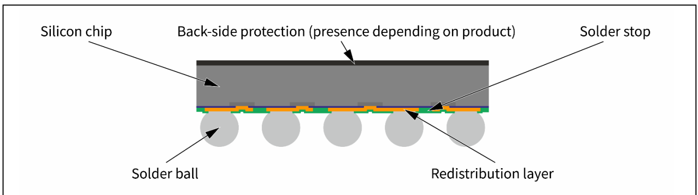
Figure 6 Schematic of the inner setup of typical WLB components.
