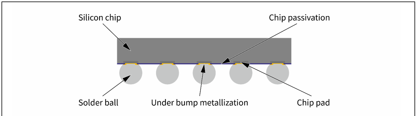
Figure 5 Schematic of the inner setup of typical WLP components.
